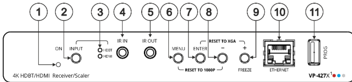
Figure 1: VP-427X1 4K HDBT/HDMI Receiver Scaler Switcher Front Panel
