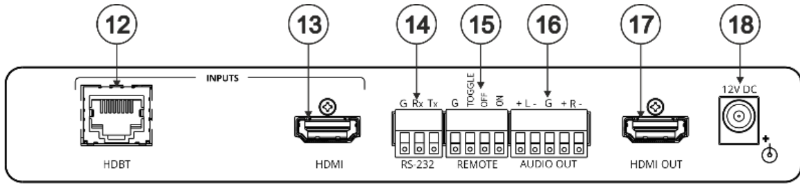
Figure 2: VP-427X1 4K HDBT/HDMI Receiver Scaler Switcher Front Panel
