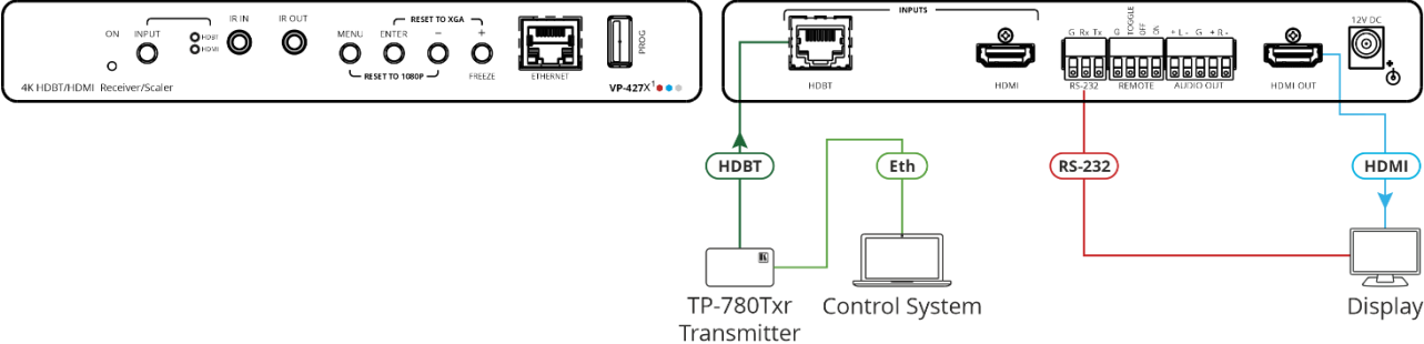
Figure 40: Ethernet Tunneling via HDBT
